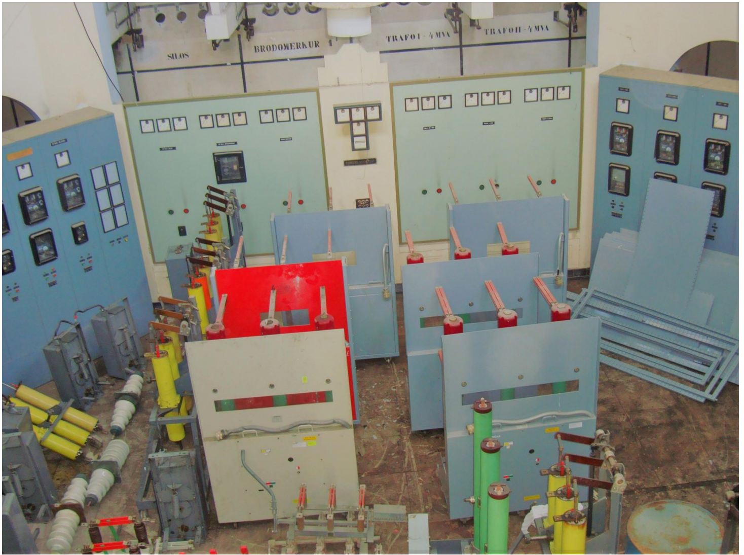
Figure A3.14: The interior of Kodl's main electrical substation.
